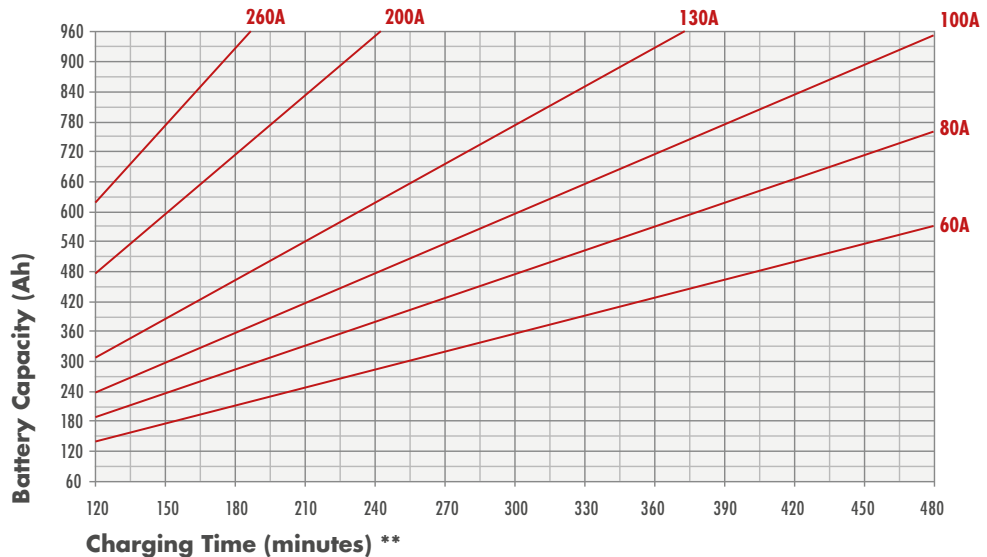
CHARGING CHARACTERISTICS* 80V (LFP 76,8V)
