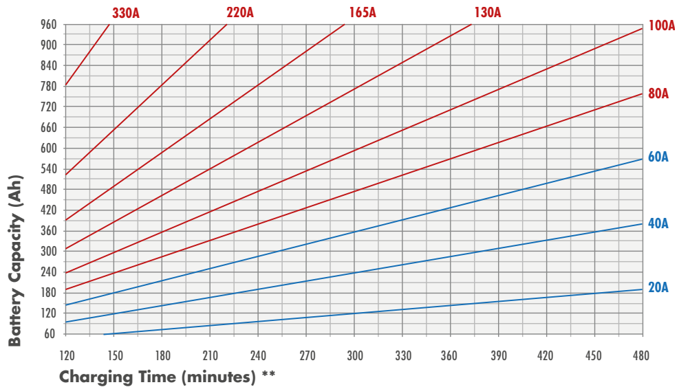
CHARGING CHARACTERISTICS* 48V (LFP 51,2V)
