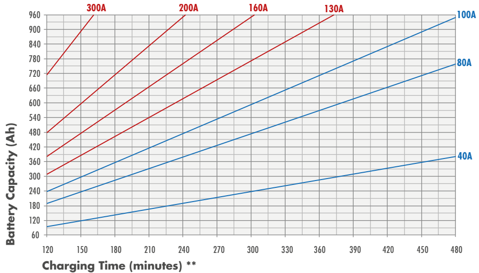
CHARGING CHARACTERISTICS* 24V (LFP 25,6V)
